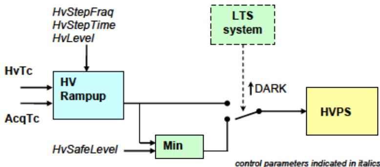
Figure 15: HVPS control signal paths
