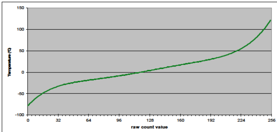
Figure 26: Temperature Conversion Curve
