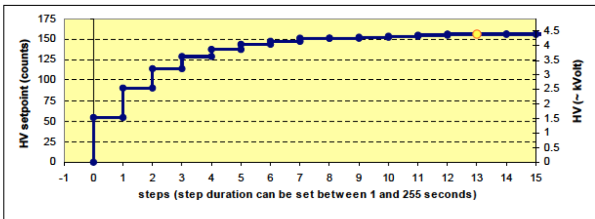
Figure 16: Example HV ramp-up from 0 to set point 157 (fraction = 45)
