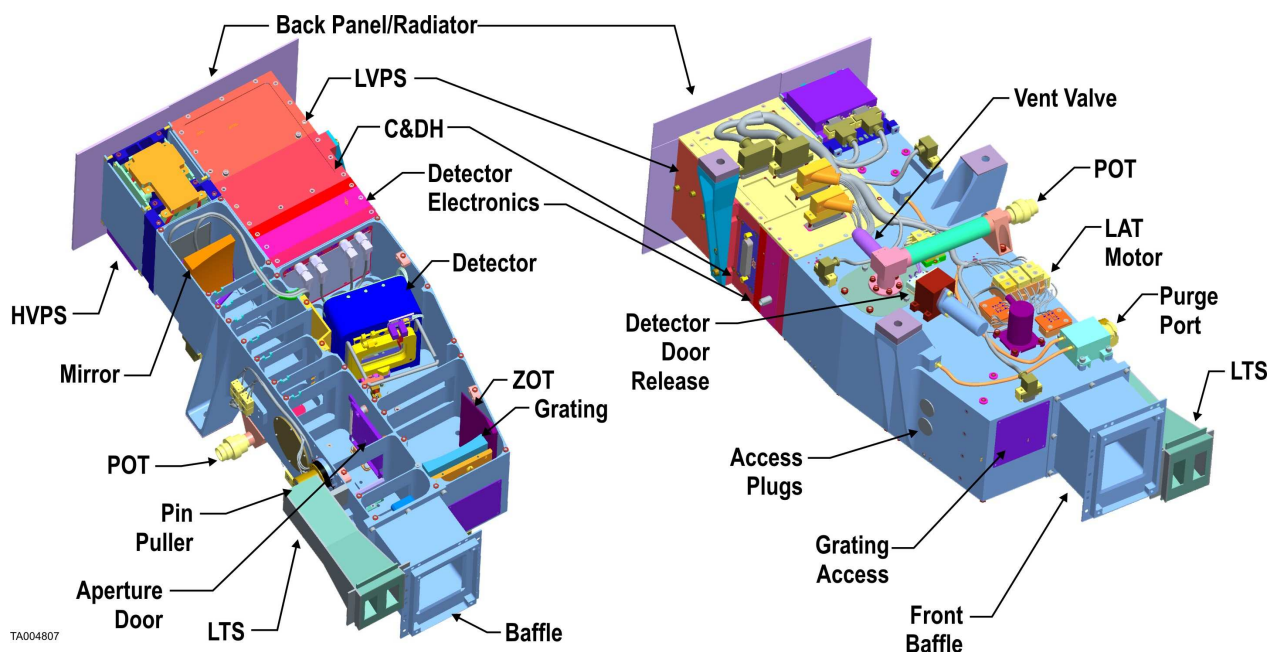
Figure 1: Three-dimensional view of LAMP with the top cover and baffle removed.
