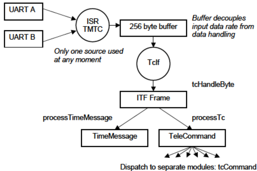
Figure 12: Command input handling
