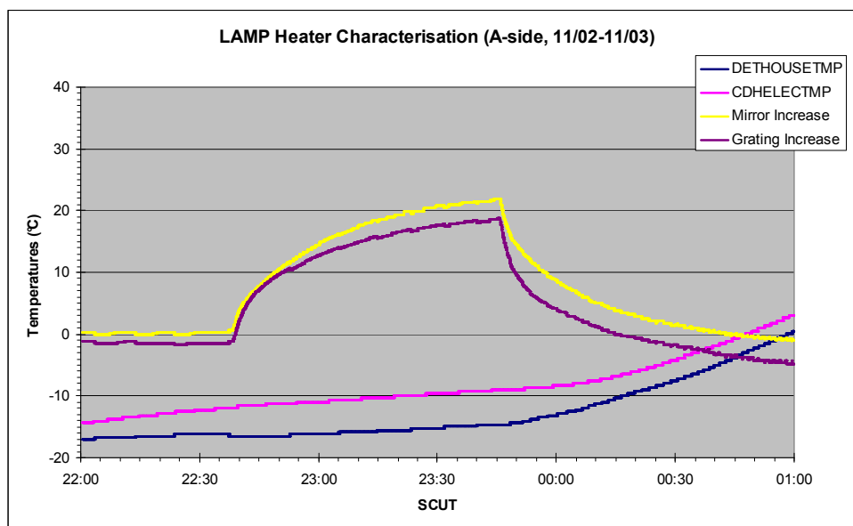
Figure 19: LAMP heater activation in vacuum, single side heaters
