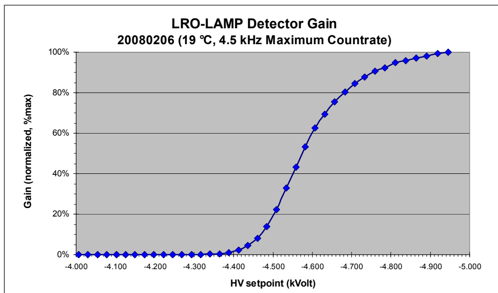
Figure 3: LAMP detector multiplication factor (gain) dependant on High Voltage
