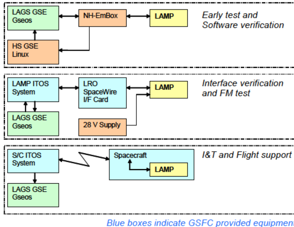
Figure 5: Test and communication configurations for the LRO-LAMP system
