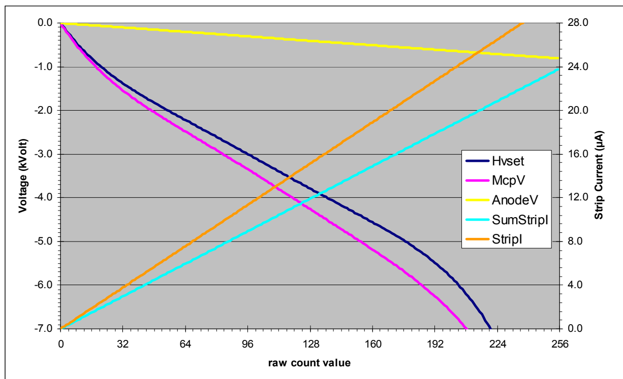
Figure 27: HVPS Parameters Conversion Curve
