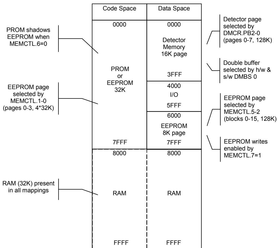
Figure 25: LAMP C&DH processor memory map
