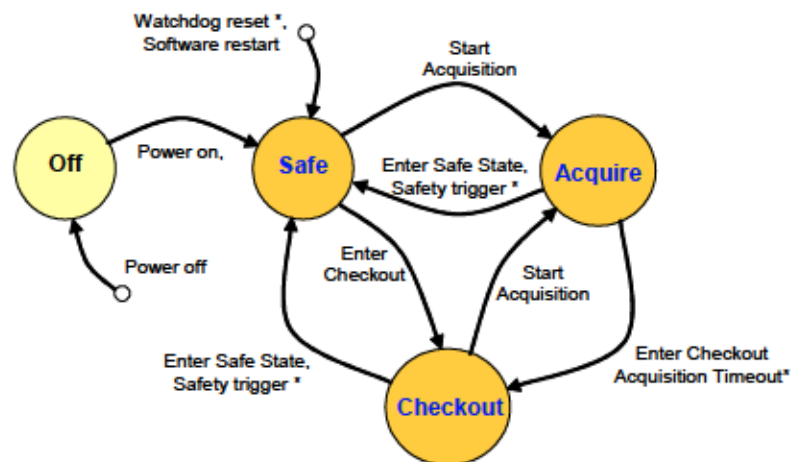
Figure 8: Operational states, state diagram
