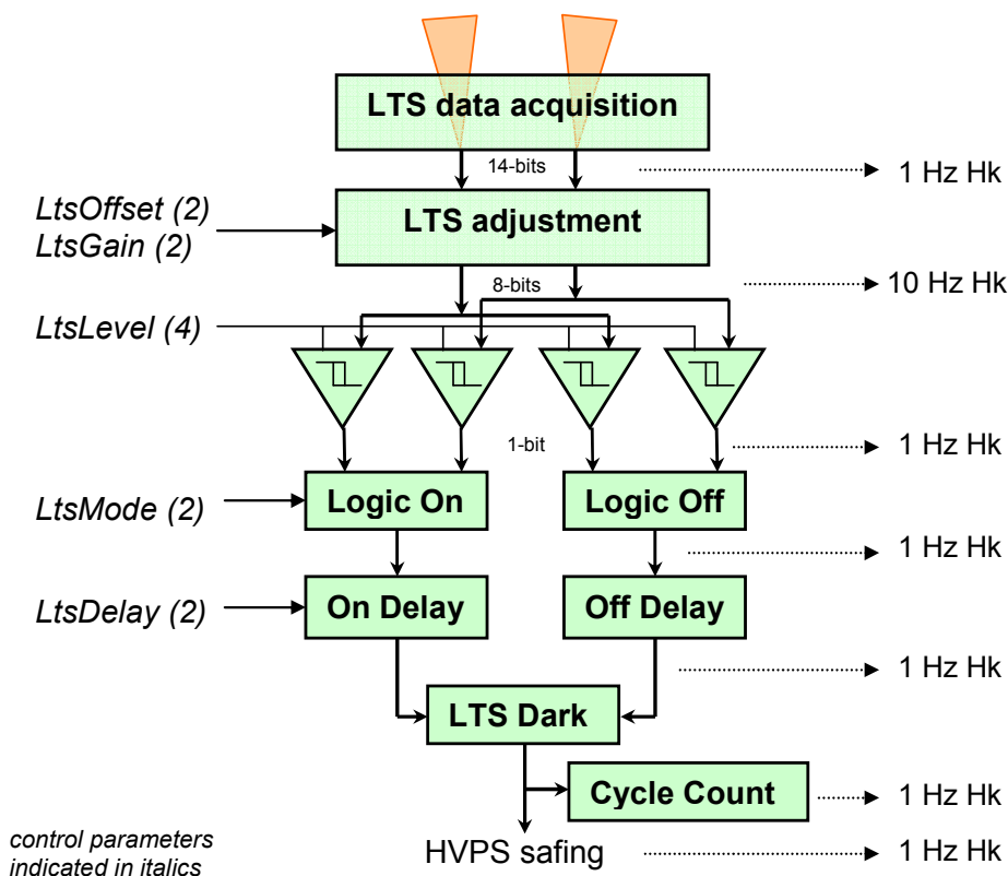
Figure 17: LTS signal processing and HK generation
