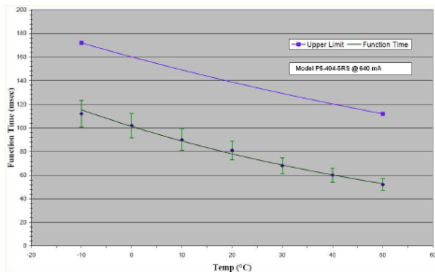
Figure 18: SMA activation times
