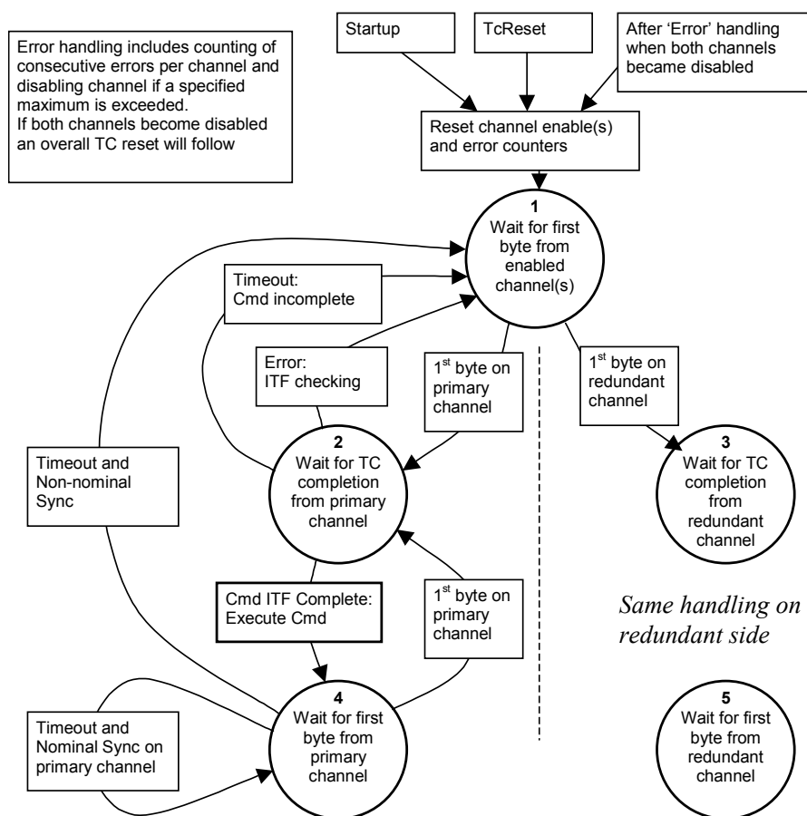
Figure 11: Primary - Secondary command processing
