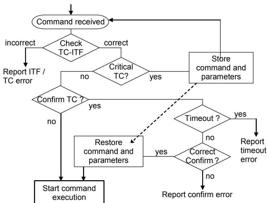
Figure 13: Critical command handling flowchart
