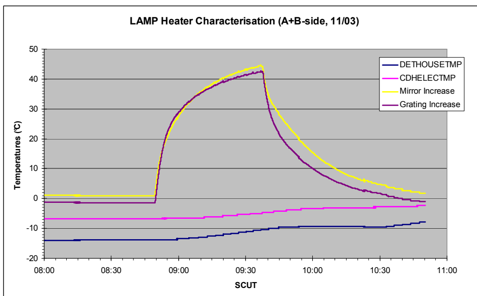
Figure 20: LAMP heater activation in vacuum, dual side heaters
