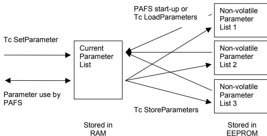
Figure 14: Parameter List storage and transfer
