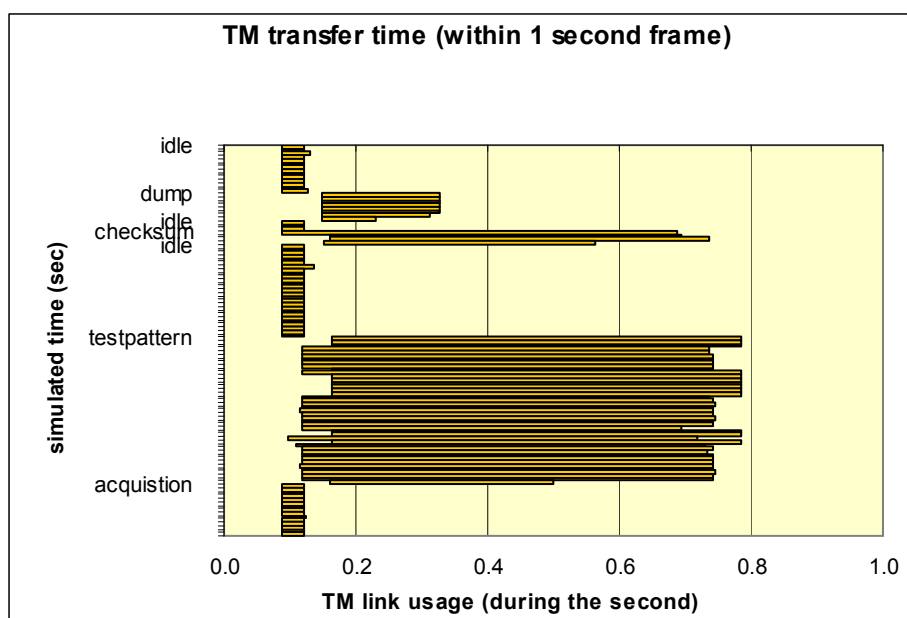
Figure 10: Simulation results: Low Speed TM transfer timing
