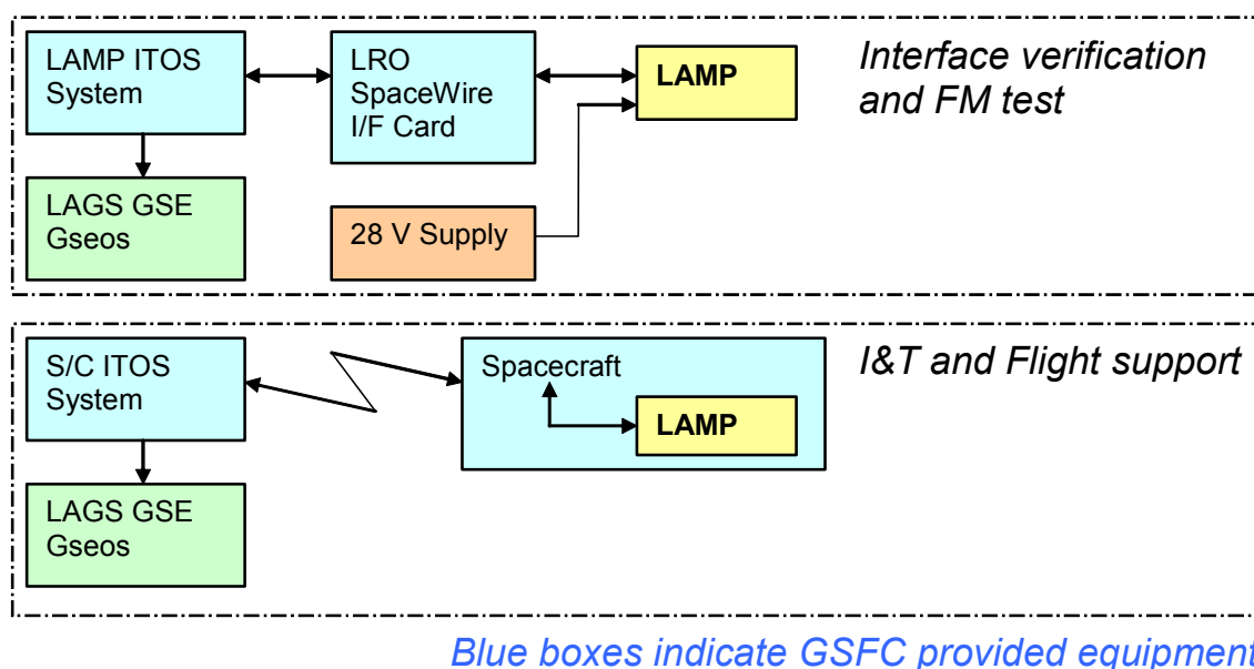
Figure 7: Overview LAMP GSE system (Engineering support, Science processing separate)
