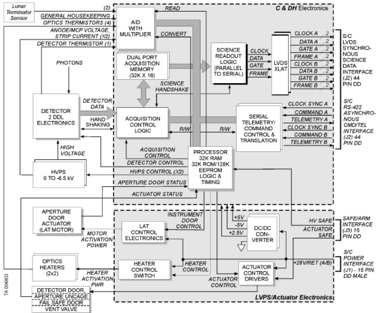
Figure 23: LAMP C&DH Electronics block diagram
