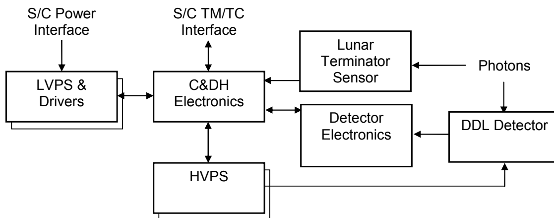
Figure 2: LAMP instrument top level electronics block diagram
