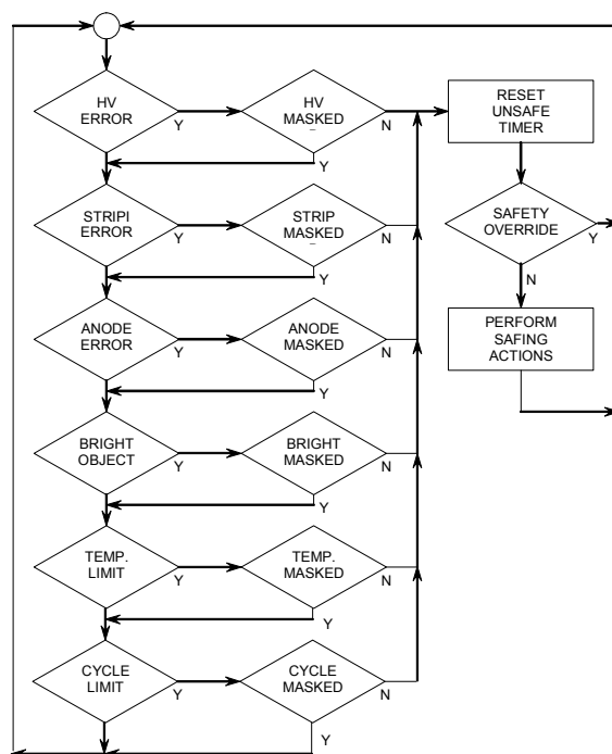
Figure 22: Safety Monitoring Algorithm Flowchart
