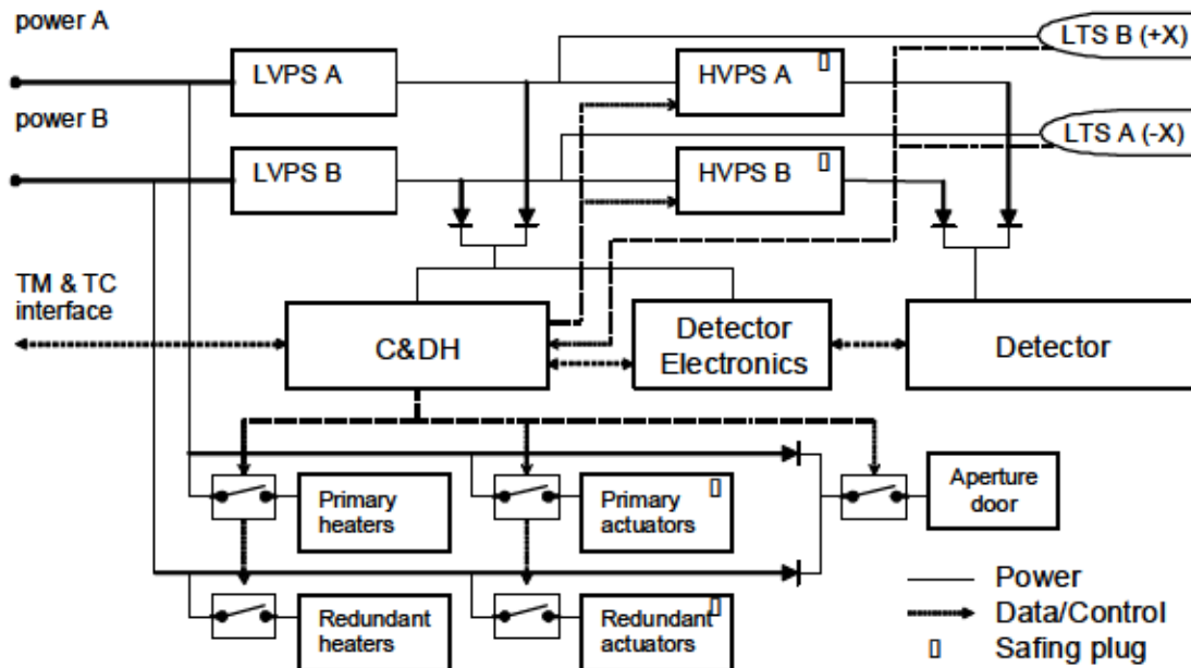
Figure 24: LAMP instrument power block diagram
