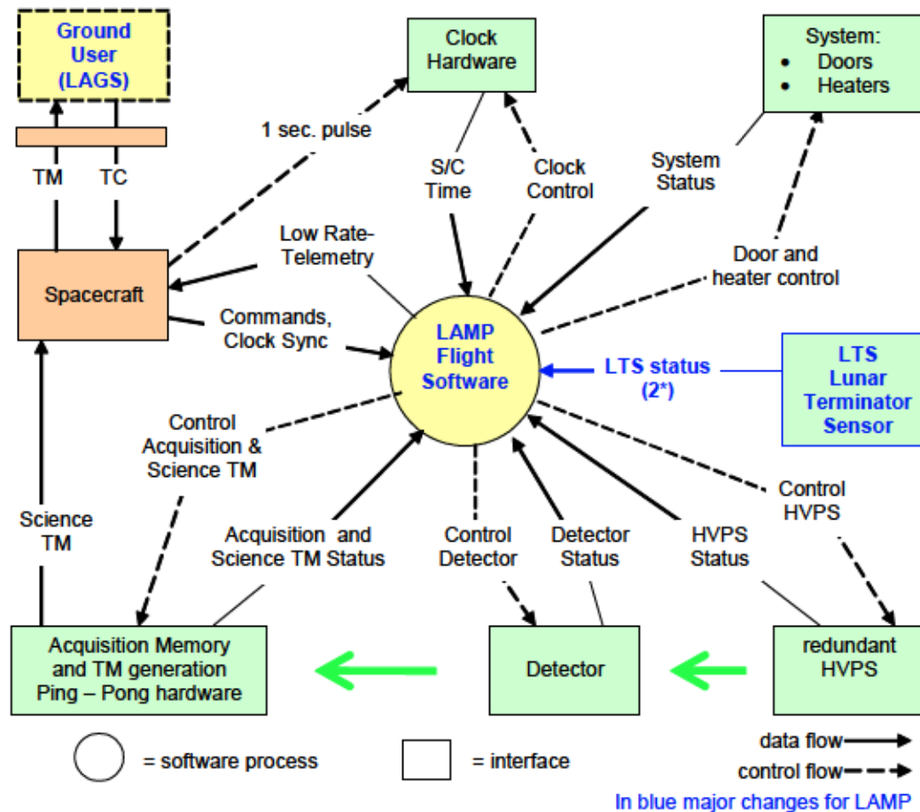
Figure 6: LRO-LAMP Flight Software Context diagram
