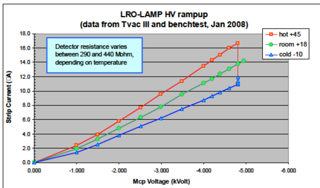
Figure 21: HVPS rampup characterization
